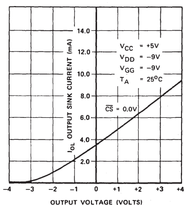
OUTPUT SINK CURRENT VS. OUTPUT VOLTAGE
